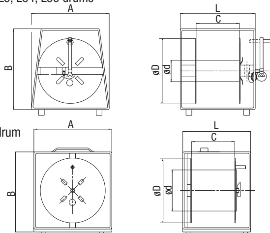
Type L2, L3, L34, L36 drums
