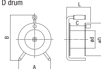
Type D drum
